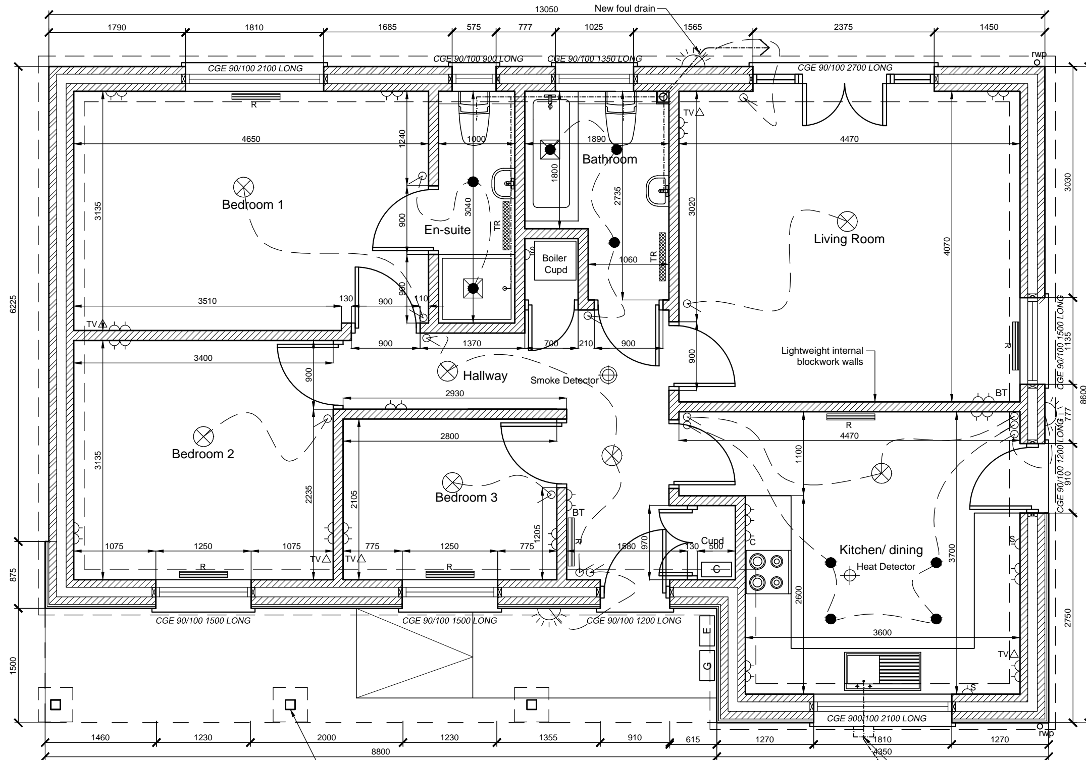
FLOOR PLAN (Plot 1) 1:50
